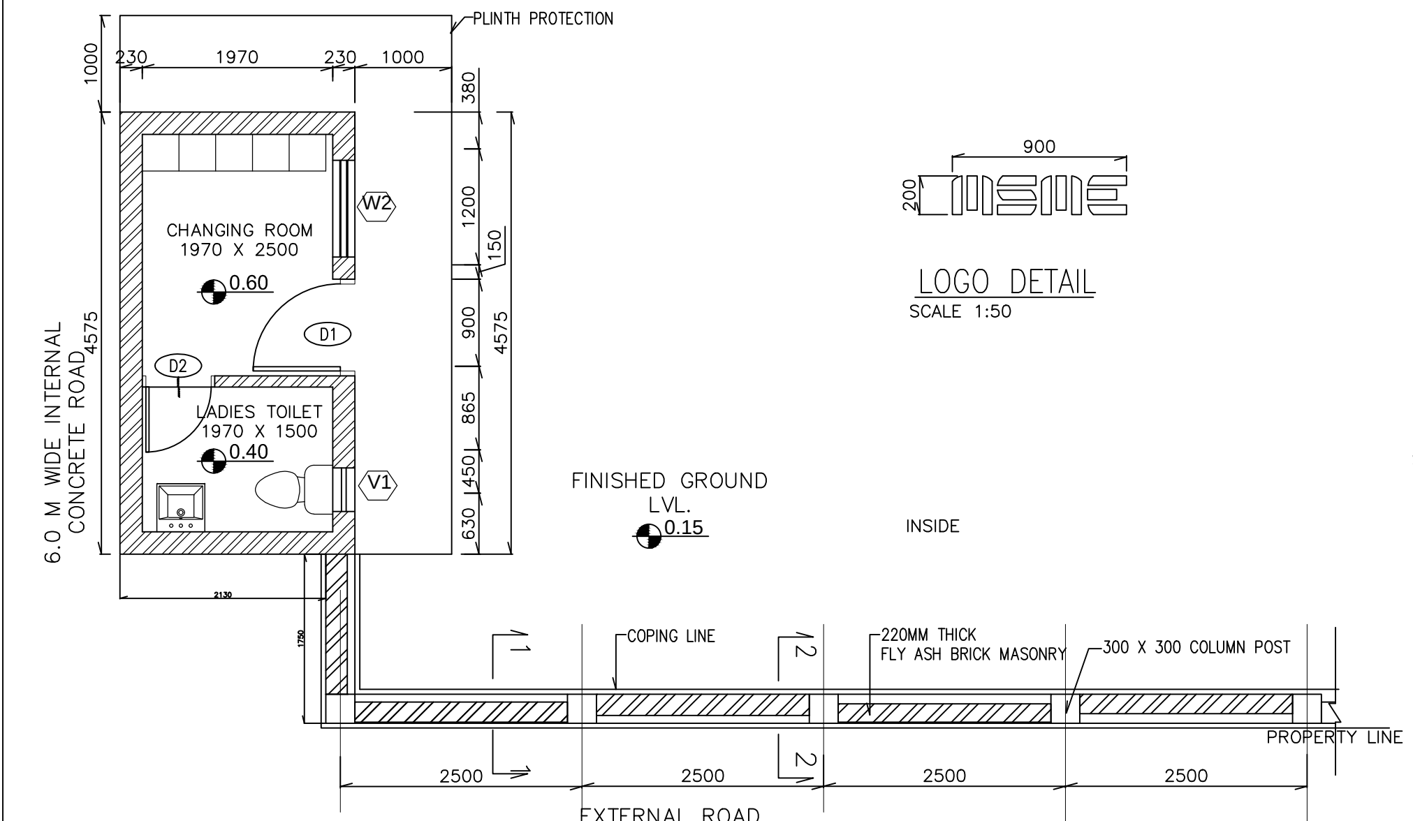
BOUNDARY WALL PLAN SCALE 1:50
